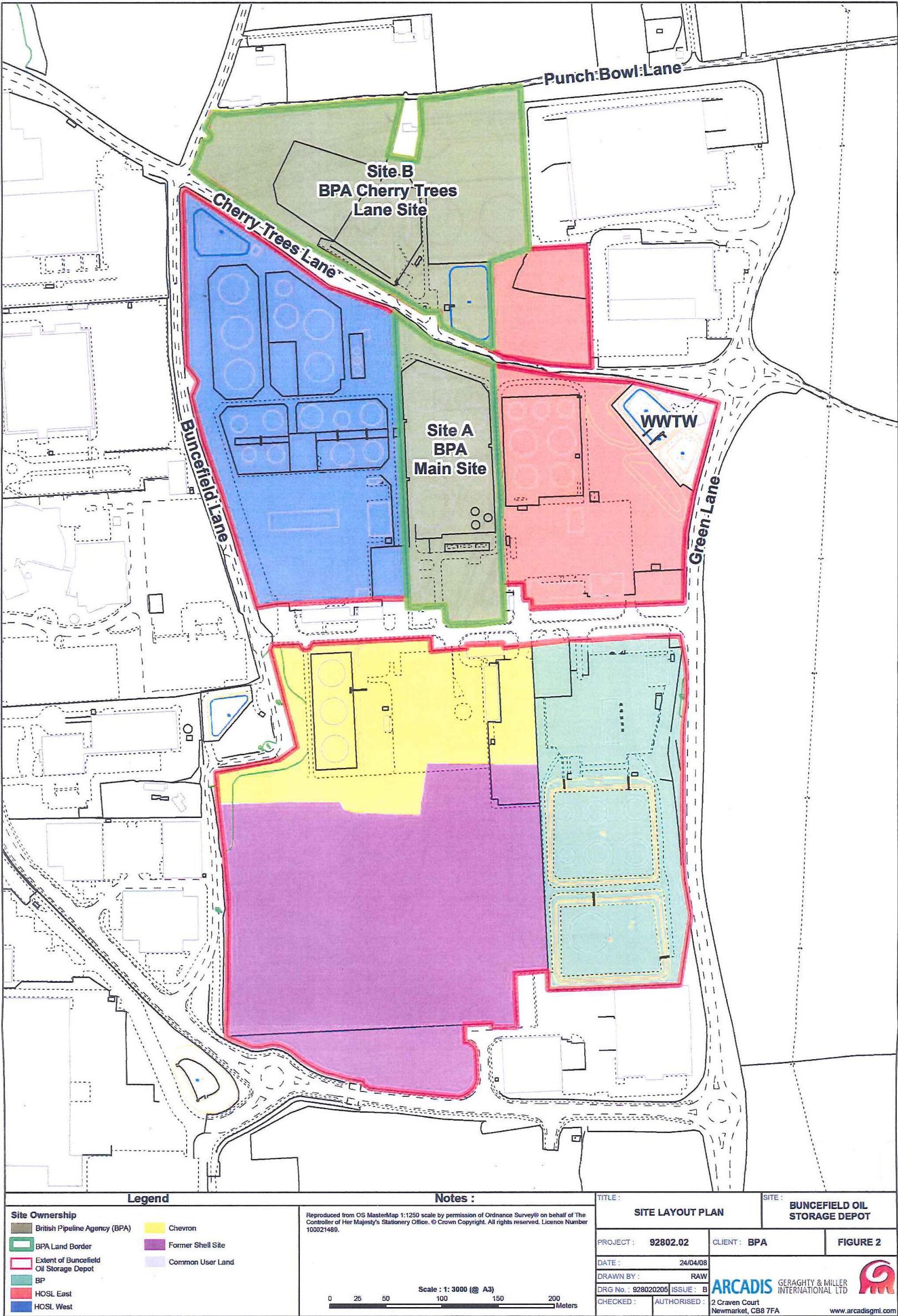
Figure D1: Site Layout and Ownership of Buncefield Oil Storage Depot (Extracted from 'WLPS & UKOP Soil Remediation Plan, Report Reference: 810530-P-RPT-061, Revision 0, 08.03.2011, Arcadis Geraghty & Miller International Ltd')
