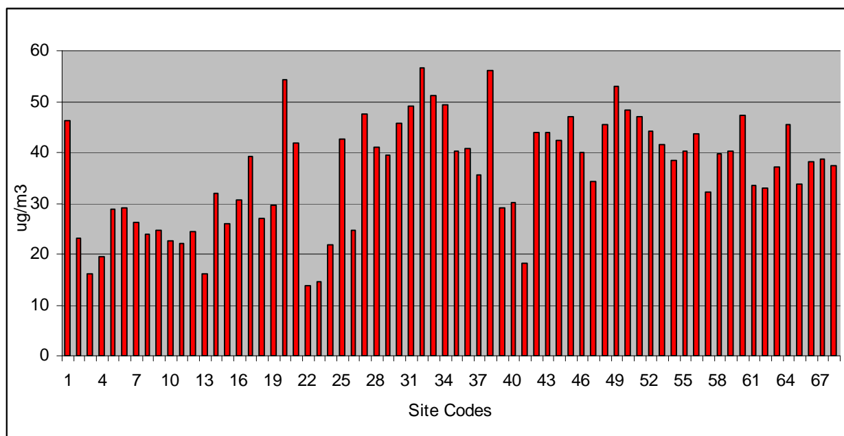
Figure 2.3 Trends in Nitrogen Dioxide Concentration Measured at Diffusion Tube Monitoring Sites.
